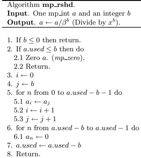
Figure 4.11: Algorithm mp_rshd
