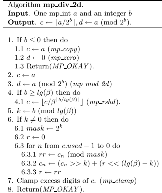
Figure 4.13: Algorithm mp_div_2d
