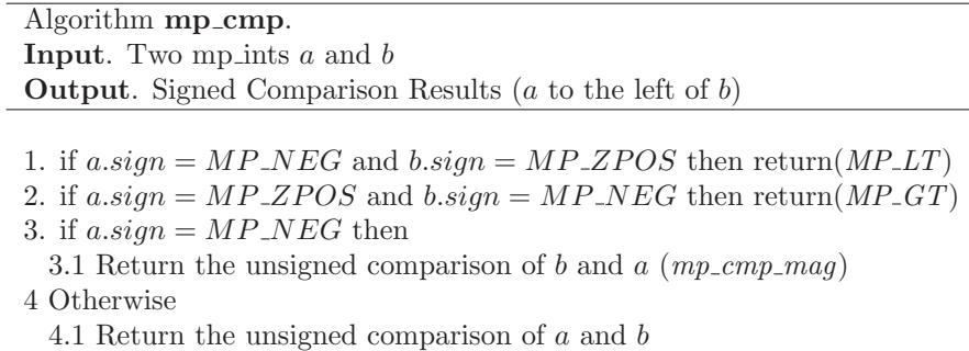
Figure 3.10: Algorithm mp_cmp
