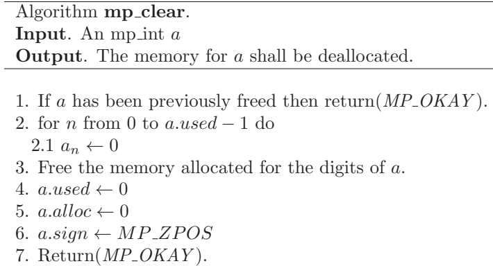
Figure 2.5: Algorithm mp_clear
