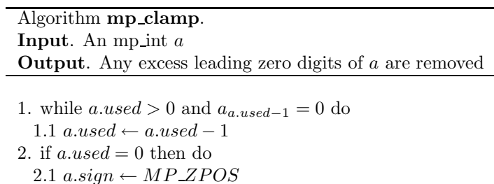
Figure 2.9: Algorithm mp_clamp
