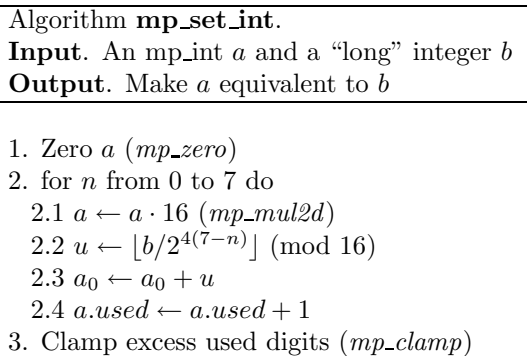
Figure 3.7: Algorithm mp_set_int
