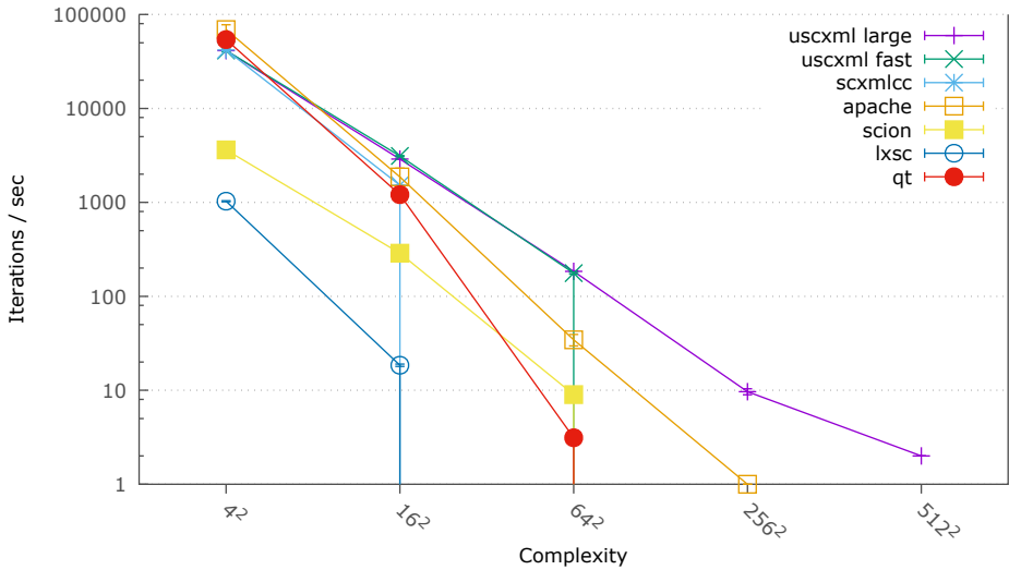
Iterations per second for LCCA Benchmark
