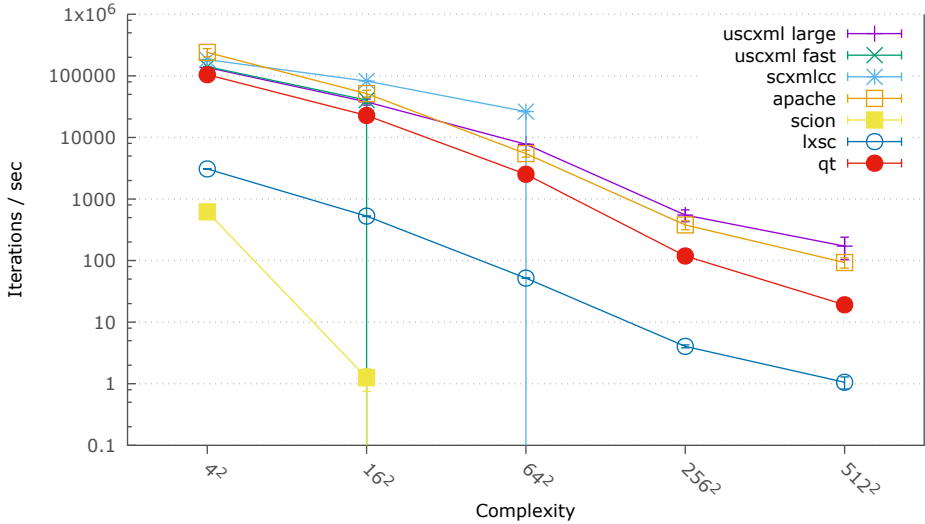
Iterations per second for Transitions Benchmark
